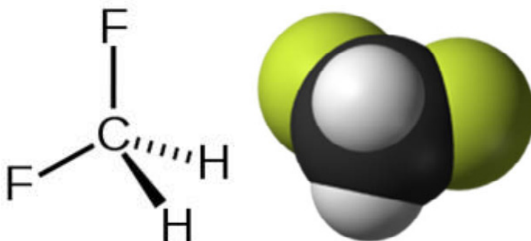
Difluoromethane
